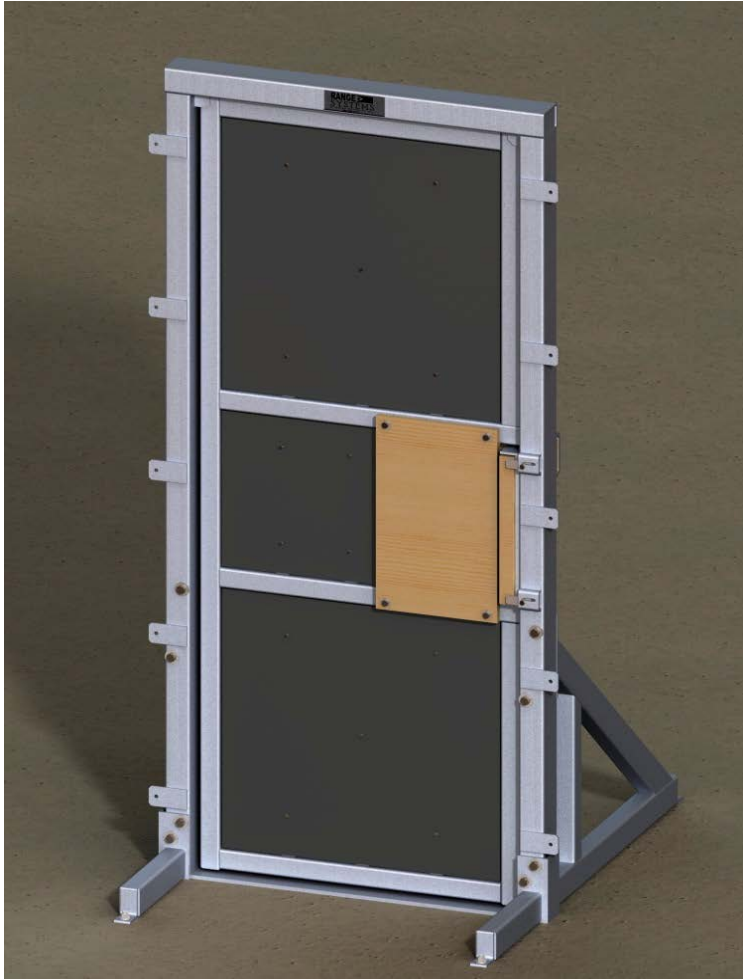
The strike plate attachment protects the door from damage and provides a realistic response when hit during ram training.
