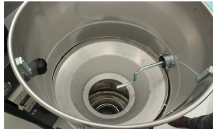
Side Mounted Manual Filter Shaker (Internal View)
